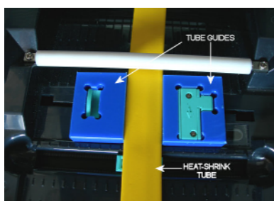
Q-LSTGUIDE in use with heat-shrink tube
